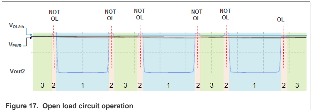
Figure 17. Open load circuit operation During normal operation, the result of the open load detection window is held until the end of the next detection window. Open load detected in the active mode is a dynamic status which is only cleared by detecting the load is not open or leaving Normal mode.
